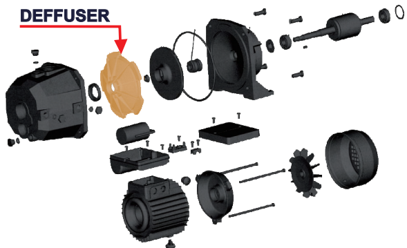
DEFFUSER GS 250
